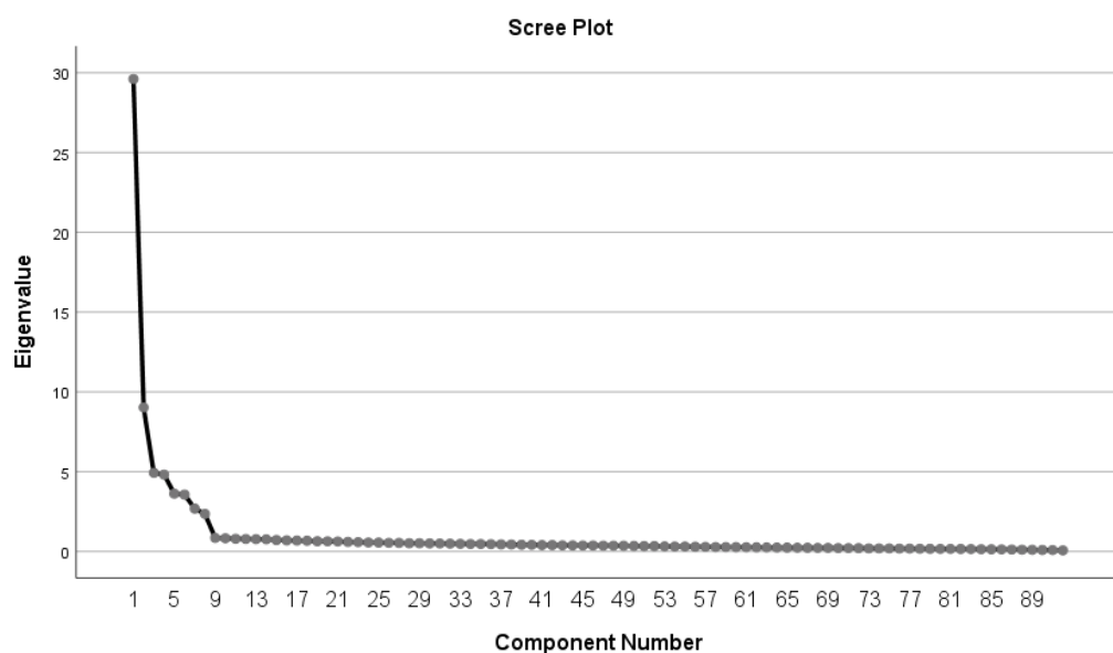
Figure 5 Scree plot
